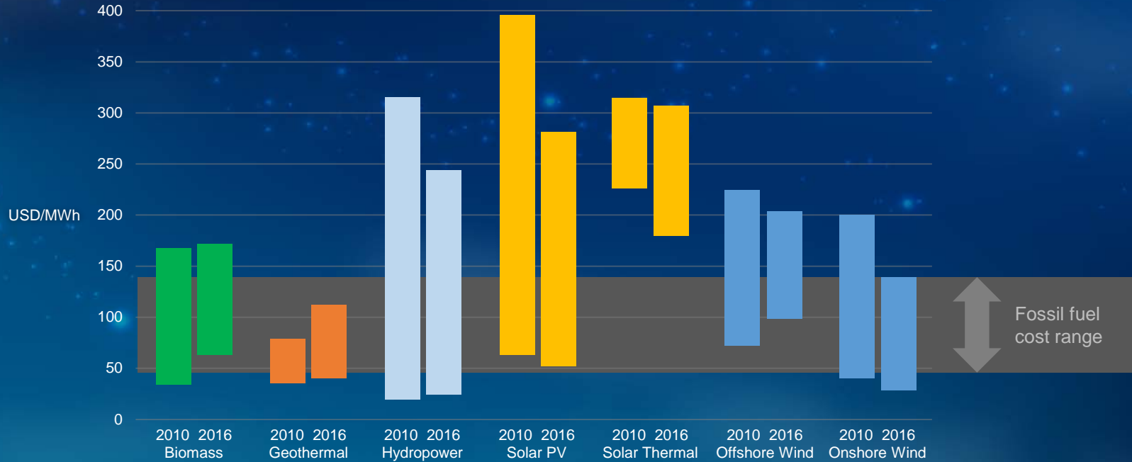
Levelised Cost of Electricity for Utility-scale Power, 2010 and 2016
